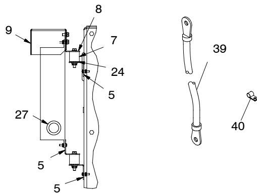
DETAIL D VIEWED FROM LEFT SIDE OF GENSET)
