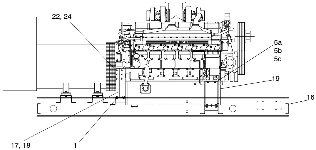
Isolation Mounting
