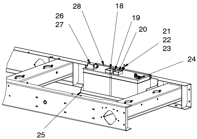
VIEW B 24V BATTERY ASSEMBLY DETAIL
