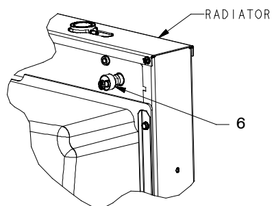
SENDER DETAIL (RIGHT SIDE VIEW)
