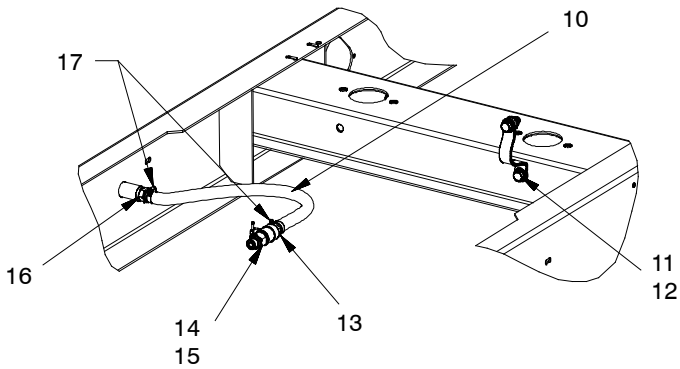
OIL DRAIN HOSE / GROUND STRAP ASSEMBLY DETAIL
