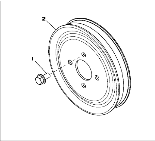
Engine Model 4024/5030
