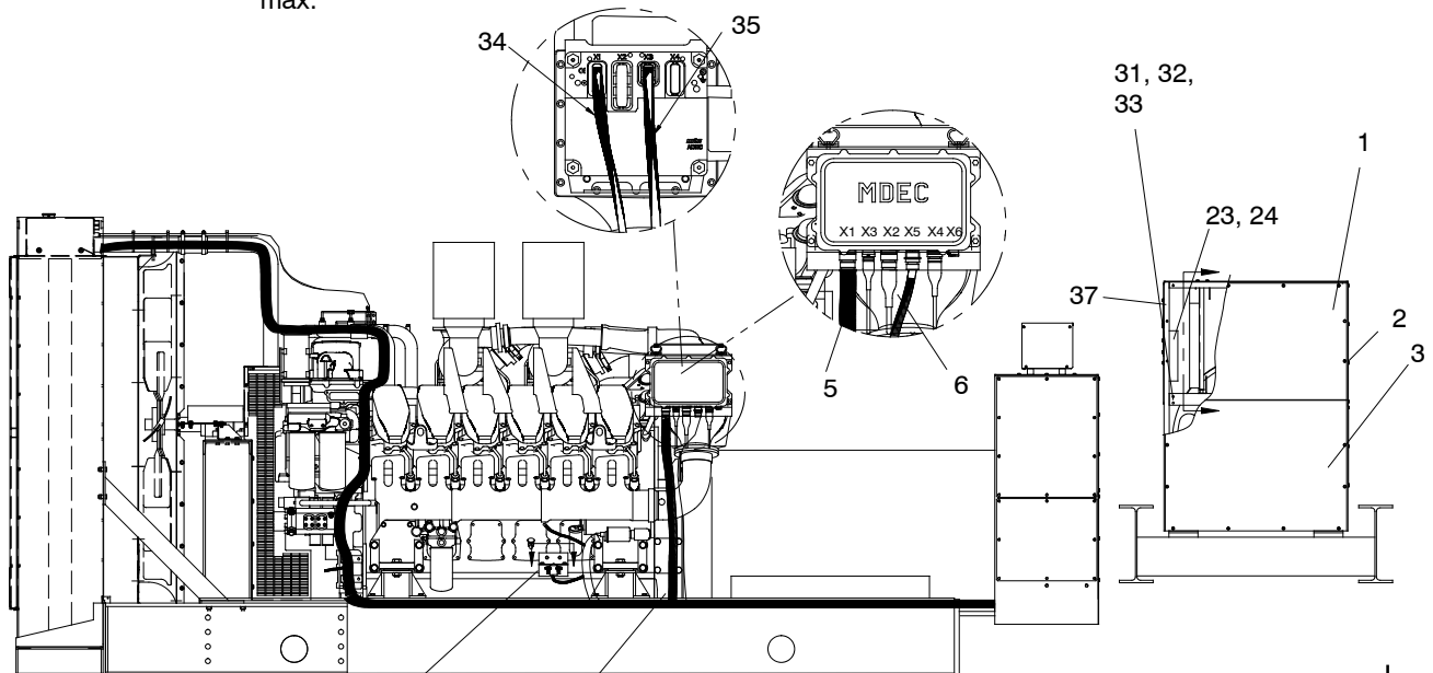
DEC 550, medium voltage
