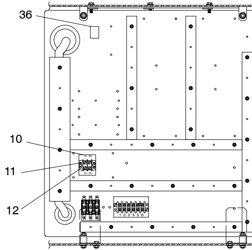
DEC 550, medium voltage
