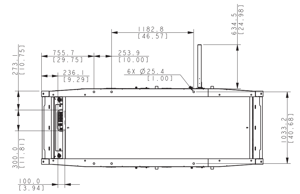
ENCLOSURE BOTTOM VIEW TANK VIEW REMOVED FOR CLARITY
