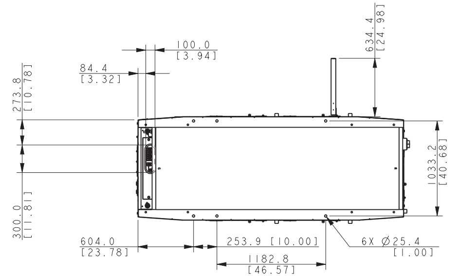
ENCLOSURE BOTTOM VIEW TANK VIEW REMOVED FOR CLARITY
