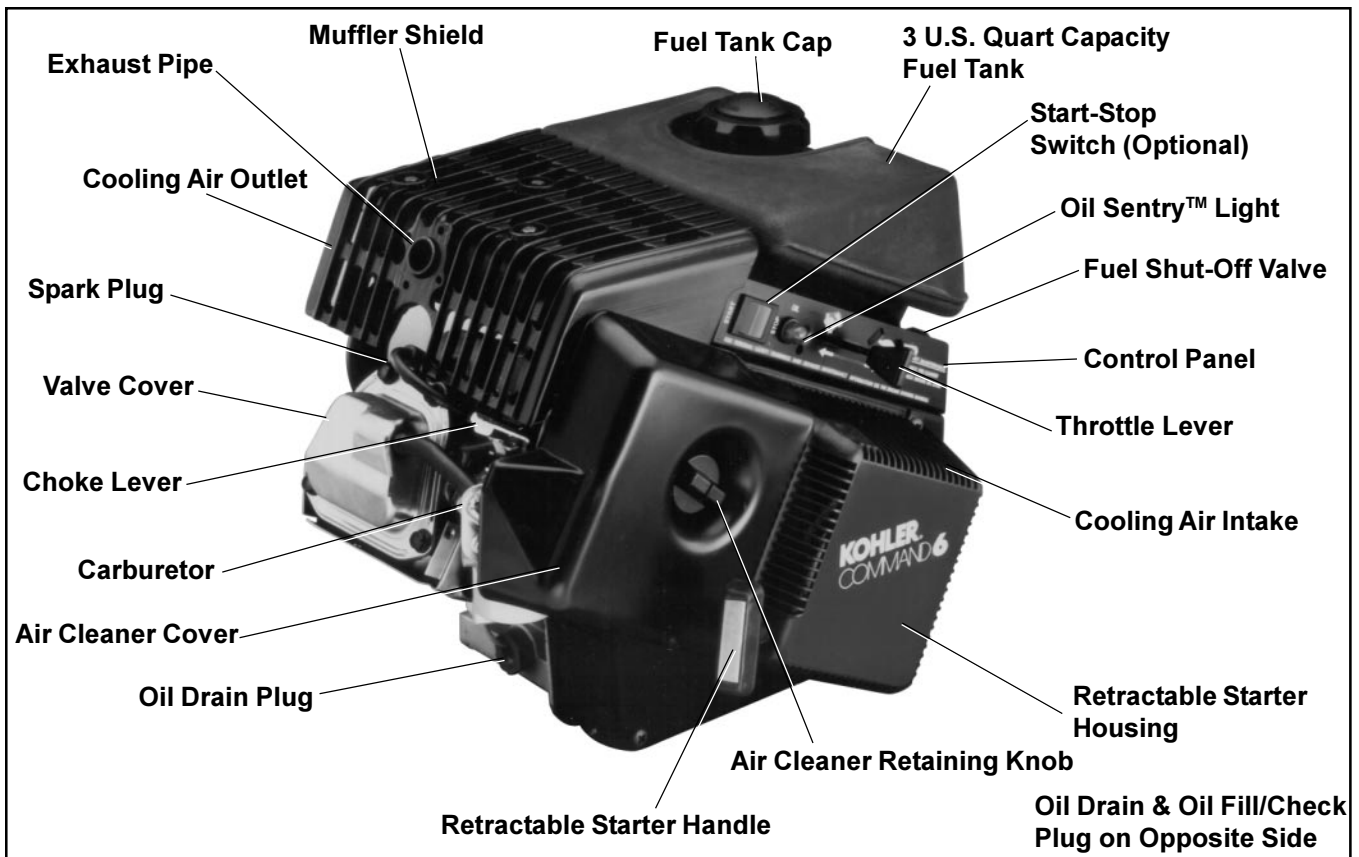
Figure 1. Location of Controls and Service Points on C6.
