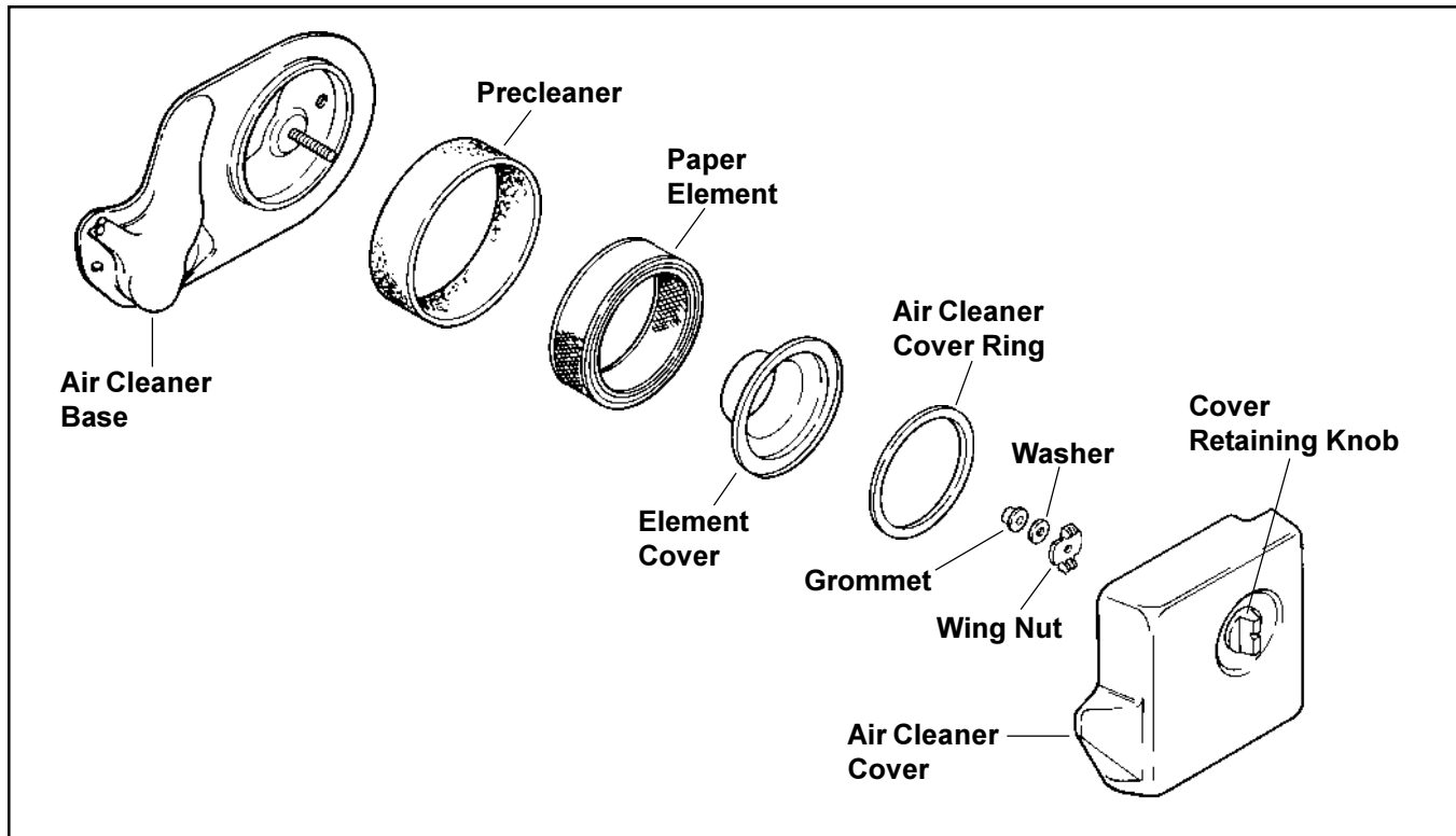
Figure 9. Air Cleaner Elements.
