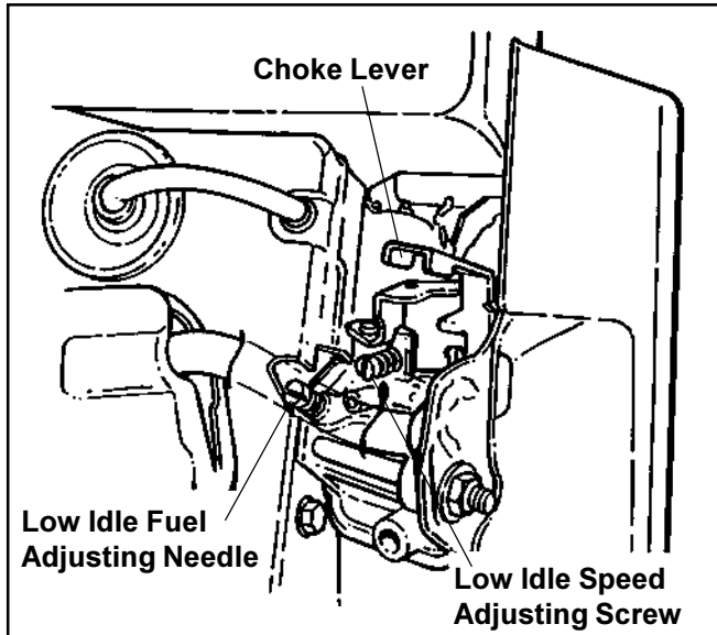
Figure 11. Fixed Main Jet Carburetor.
