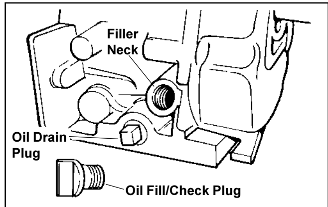
Figure 7. Location of Oil Drain and Check Plugs.
