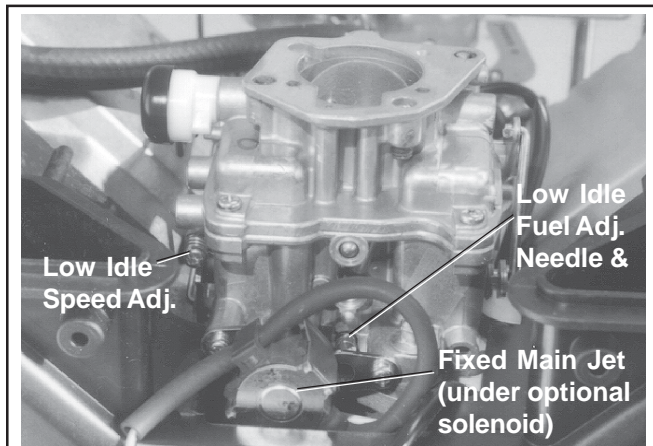
Figure 17. Carburetor (CH18-23, CH620-CH730, CH740).
