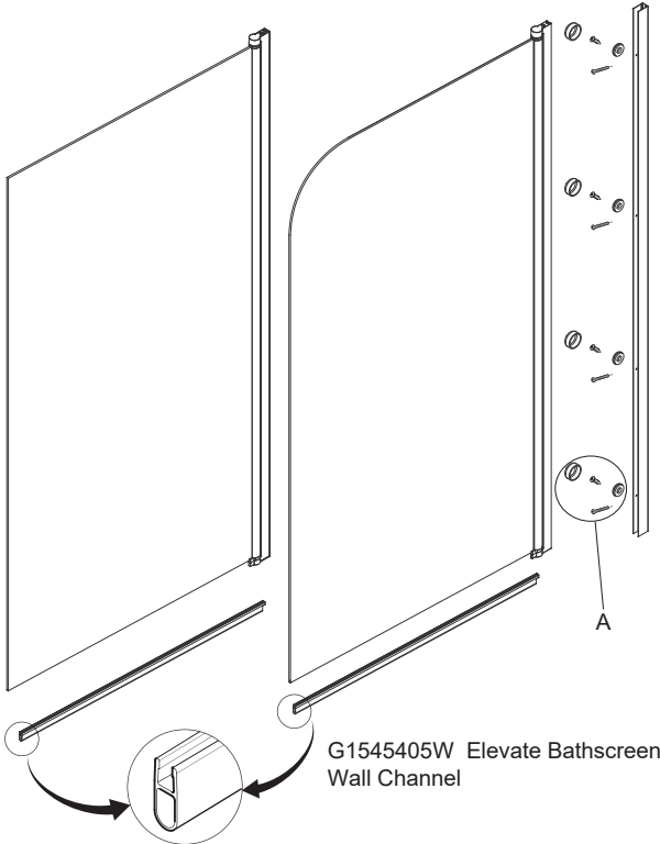
G1545405W Elevate Bathscreen Wall Channel
