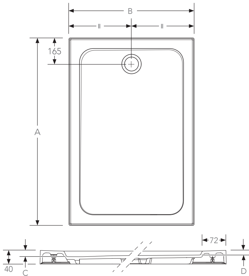
Side Profile of Non-Upstand Tray
