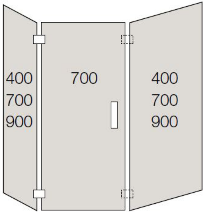
1400 x 900 mm
