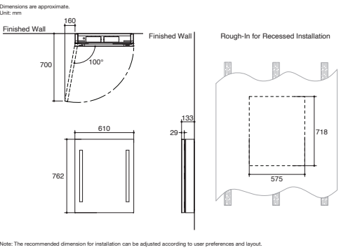
New Verdera 610 mm Mirrored Cabinet with Lights and Defogger K-78202X-L-NA • Overall dimensions 610 x 133 x 762 mm. • For recessed or surface-mount installation.
