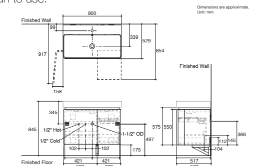
Aleutian 900 mm Bathroom Cabinet K-45764X-0 • Overall dimension 892 x 517 x 575 mm.
