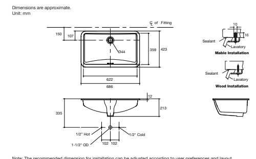
Ladena 27" Undercounter Lavatory K-76509K-0 • Overall dimension 686 x 423 x 213 mm. • With overflow.
