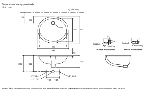
Caxton 17" Undercounter Lavatory K-2210X-0 • Overall dimension 489 x 413 x 191 mm. • With overflow.
