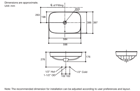
ModernLife Vessel Lavatory K-77762X-0 (No faucet hole) • Overall dimensions 598 x 397 x 176 mm • With overflow.
