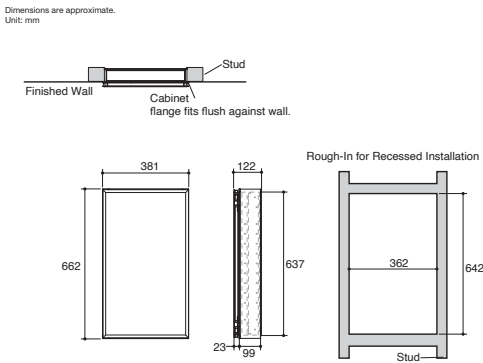
Elosis 381 mm Mirrored Cabinet K-15030T-NA • Overall dimensions 381 x 122 x 662 mm. • For surface-mount installation.
