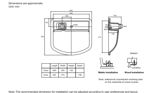
Family Care Undercounter Lavatory K-21916T-1-0 (Single Hole) • Overall dimension 620 x 555 x 193 mm. • Without overflow. • Non Stock Item.
