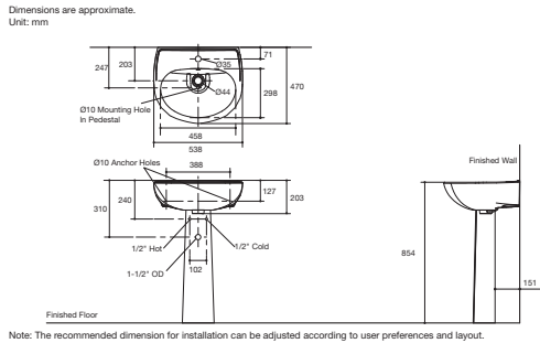
Sacramento Pedestal Lavatory K-8703X-1-0 (Single Hole) K-8705X-0 (Pedestal) • Overall dimension 538 x 470 x 854 mm. • With overflow.
