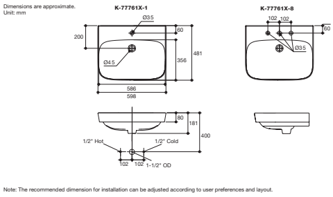
ModernLife Vessel Lavatory K-77761X-1-0 (Single Hole) K-77761X-8-0 (8" Center) • Overall dimensions 598 x 481 x 181 mm • With overflow.
