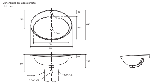
Karess Self-Rimming Lavatory K-2759X-1-0 (Single Hole) • Overall dimension 615 x 443 x 197 mm. • With overflow.
