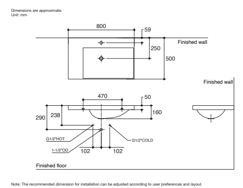
Toobi 800 mm Vanity Top K-45471X-ZW-0 Overall dimension 800 x 500 x 160 mm.
