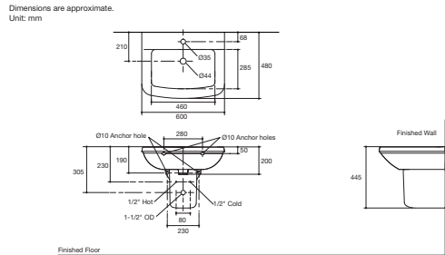
Panache Semi-Pedestal Lavatory K-17156X-0 (Single Hole) K-17154X-0 (Semi-Pedestal) • Overall dimension 600 x 480 x 445 mm. • With overflow.
