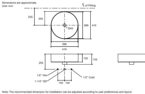
Mica Round Vessel Lavatory K-90012X-0 (No faucet hole) • Overall dimension 410 x 410 x 155 mm. • Without overflow.
