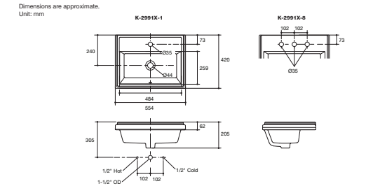
Tresham Self-Rimming Lavatory K-2991X-1-0 (Single Hole) K-2991X-8-0 (8" Center) • Overall dimensions 554 x 420 x 205 mm. • With overflow.
