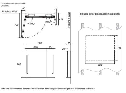
New Verdera 866 mm Mirrored Cabinet with Lights and Defogger K-78282X-NA • Overall dimensions 866 x 133 x 762 mm. • For recessed or surface-mount installation.
