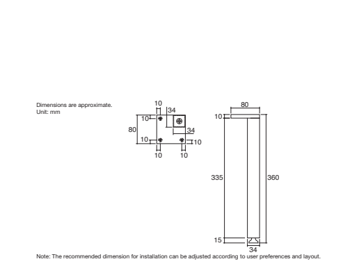
Feet for Toobi Bathroom Furniture K-45405X-NA Overall dimension 80 x 80 x 360 mm. 2 pieces per package.
