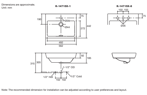
Parliament Vessel Lavatory K-14715X-1-0 (Single Hole) K-14715X-8-0 (8" Center) • Overall dimension 562 x 442 x 185 mm. • With overflow.
