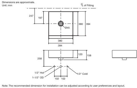
Mica Square Vessel Lavatory K-90011X-0 (No faucet hole) • Overall dimension 394 x 394 x 158 mm. • Without overflow.
