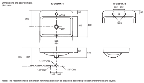
Forefront Rectangular Vessel Lavatory K-2660X-1-0 (Single Hole) K-2660X-8-0 (8" Center) • Overall dimension 584 x 460 x 173 mm. • With overflow.
