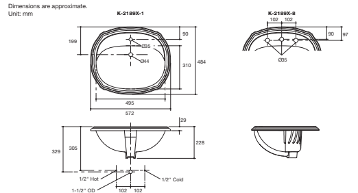
Portrait Self-Rimming Lavatory K-2189X-1-0 (Single Hole) K-2189X-8-0 (8" Center) • Overall dimension 572 x 484 x 228 mm. • With overflow.
