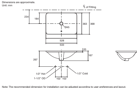
Carillon Rectangular Vessel Lavatory K-96117X-0 (No faucet hole) • Overall dimension 533 x 368 x 167 mm. • With overflow.
