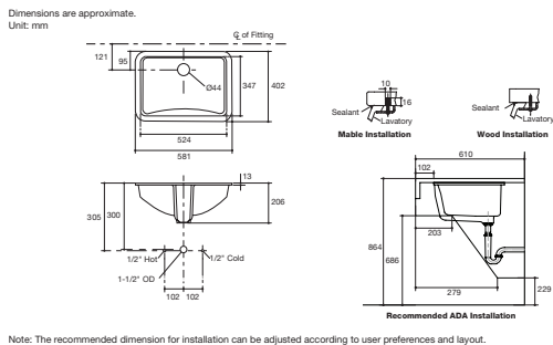
Ladena 21" Undercounter Lavatory K-2215X-0 • Overall dimension 581 x 402 x 206 mm. • With overflow.
