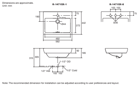
Parliament Vessel Lavatory K-14715X-1-0 (Single Hole) K-14715X-8-0 (8" Center) • Overall dimension 562 x 442 x 185 mm. • With overflow.
