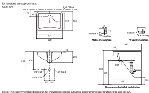
Ladena 18" Undercounter Lavatory K-2214X-0 • Overall dimension 530 x 365 x 206 mm. • With overflow.
