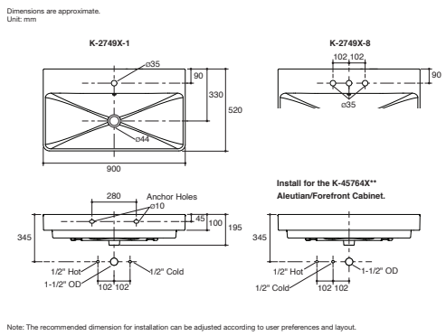
Forefront 900 mm Vanity Top K-2749X-1-0 (Single Hole) K-2749X-8-0 (8" Center) • Overall dimension 900 x 520 x 145 mm.
