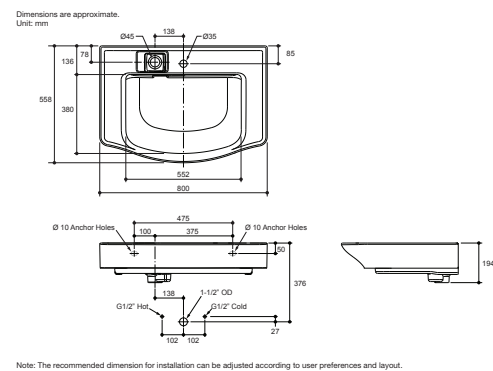
Family Care 800 mm Vanity Top K-22779X-1-0 • Overall dimesions 800 x 558 x 194 mm.
