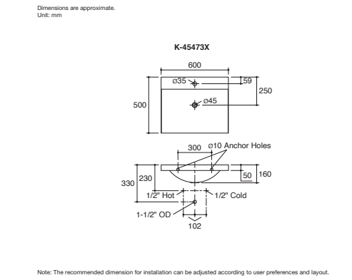
Toobi 600 mm Vanity Top K-45473X-0 Overall dimension 600 x 500 x 160 mm.
