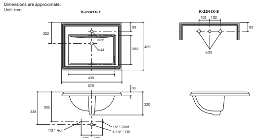
Memoirs (Classic Design) Self-Rimming Lavatory K-2241X-1-0 (Single Hole) K-2241X-8-0 (8" Center) • Overall dimension 579 x 459 x 220 mm. • With overflow.
