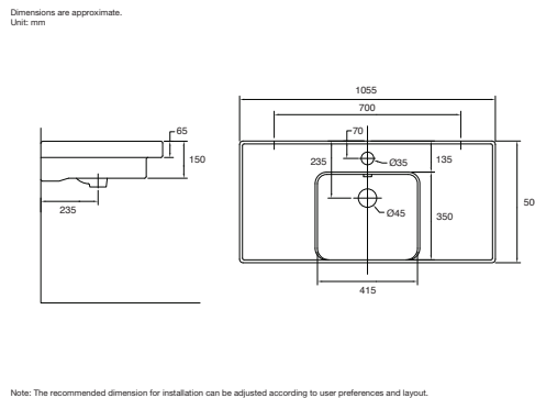
Reach 1000 mm Vanity Top K-18571T-1-0 • Overall dimension 1,055 x 500 x 510 mm.
