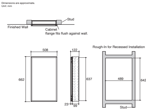
Elosis 508 mm Mirrored Cabinet K-15031T-NA • Overall dimensions 508 x 122 x 662 mm. • For surface-mount installation.
