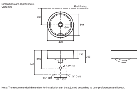
Chalice Vessel Lavatory K-14800X-0 (No faucet hole) • Overall dimension 420 x 420 x 203 mm. • With overflow.
