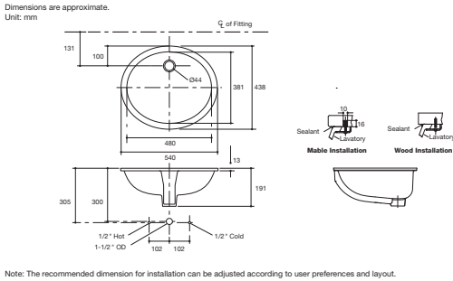
Caxton 19" Undercounter Lavatory K-2211X-0 • Overall dimension 540 x 438 x 191 mm. • With overflow.
