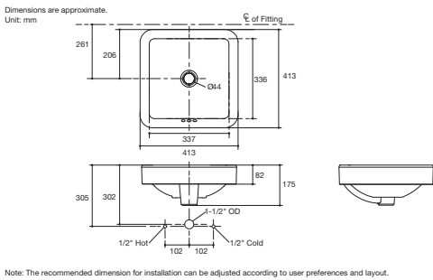
Forefront Square Vessel Lavatory K-2661X-0 (No faucet hole) • Overall dimension 413 x 413 x 175 mm. • With overflow.
