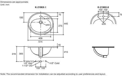
Pennington Self-Rimming Lavatory K-2196X-1-0 (Single Hole) K-2196X-8-0 (8" Center) • Overall dimension 514 x 445 x 215 mm. • With overflow.
