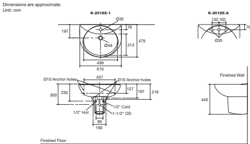
Folio Semi-Pedestal Lavatory K-2018X-1-0 (Single Hole) K-2018X-8-0 (8" Center) K-11340X-0 (Semi-Pedestal) • Overall dimension 610 x 479 x 440 mm. • With overflow.
