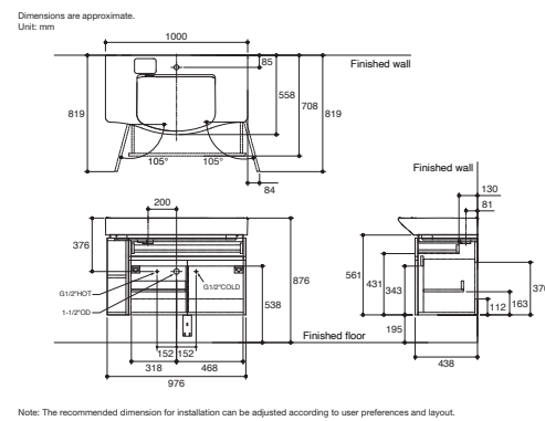
Family Care 1000 mm Bathroom Cabinet K-31503X-L-PD1 • Overall dimesions 976 x 438 x 540 mm. • Left open storage shelves.
