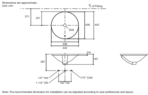
Carillon Round Vessel Lavatory K-96118X-0 (No faucet hole) • Overall dimension 442 x 442 x 167 mm. • With overflow.
