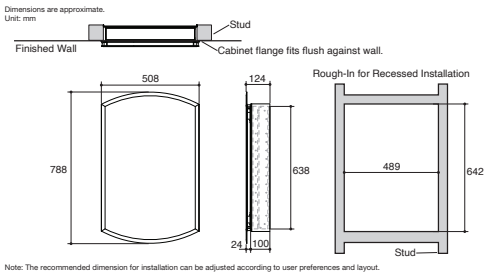
Archer Mirrored Cabinet K-3073T-NA • Overall dimensions 508 x 124 x 788 mm. • For recessed or surface-mount installation.
