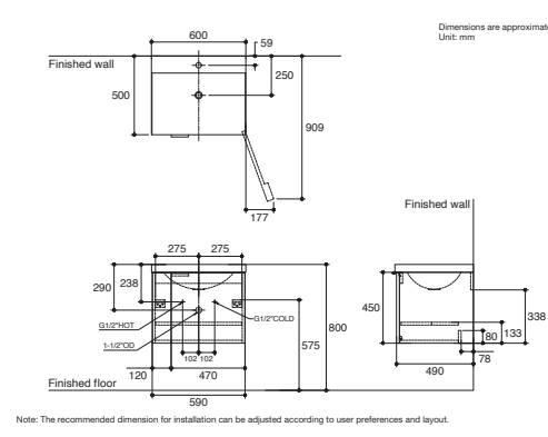
Toobi 600 mm Bathroom Cabinet K-45472X-BWP Overall dimension 590 x 490 x 450 mm.
