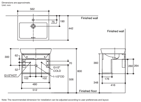
Regatta Hydroshield Plain 500 mm for 14715X Bathroom Cabinet K-31092X-GSK • Overall dimension 512 X 416 X 360 mm.
