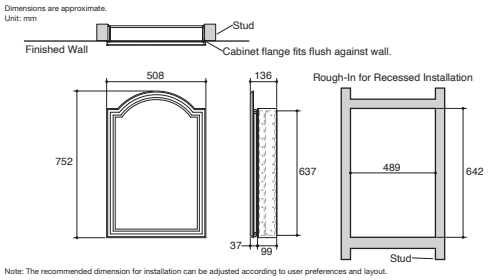
Devonshire Mirrored Cabinet K-15035T-NA • Overall dimensions 508 x 136 x 752 mm. • For recessed or surface-mount installation.
