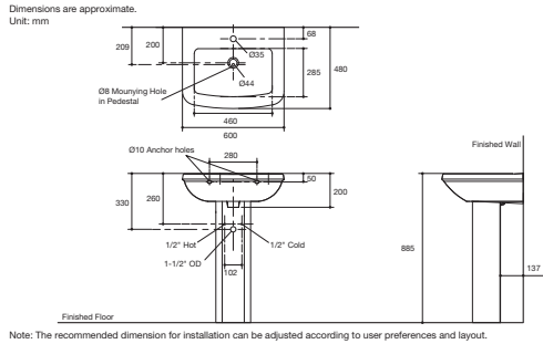
Panache Pedestal Lavatory K-17156X-0 (Single Hole) K-17153X-0 (Pedestal) • Overall dimension 600 x 480 x 885 mm. • With overflow.
