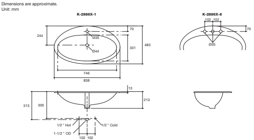
Ellipse Self-Rimming Lavatory K-2886X-1-0 (Single Hole) K-2886X-8-0 (8" Center) • Overall dimension 838 x 483 x 213 mm. • With overflow. • Made from Cast Iron.
