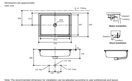
Verticyl Undercounter Lavatory K-2889X-UDL-0 • Overall dimension 575 x 420 x 178 mm. • With overflow.
