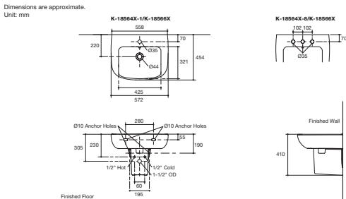
Reach Semi-Pedestal Lavatory K-18564X-1-0 (Single Hole) K-18564X-8-0 (8" Center) K-18566X-0 (Semi-Pedestal) • Overall dimension 572 x 454 x 410 mm. • With overflow.
