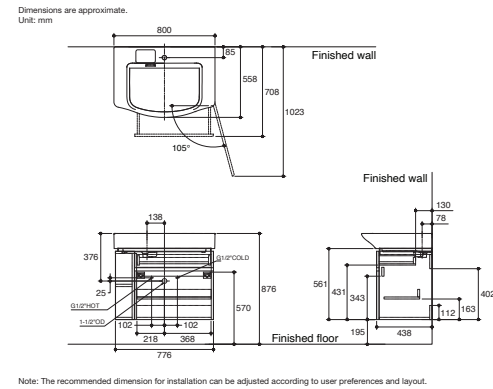
Family Care 800 mm Bathroom Cabinet K-31501X-L-PD1 • Overall dimesions 776 x 438 x 540 mm. • Left open storage shelves.
