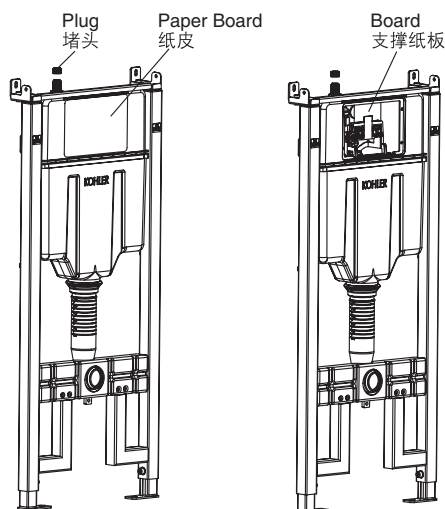
In-wall Tank With Frame 入墙式隐藏水箱(含固定支架)座便器
