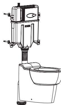
In-wall Tank Without Frame 入墙式隐藏水箱(不含固定支架)座便器
