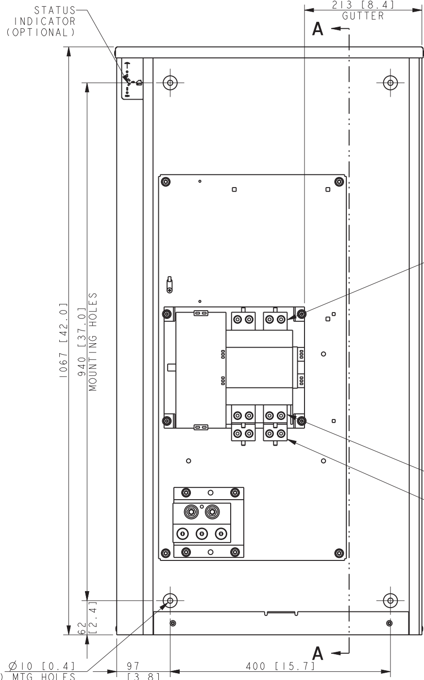
400A CONTACTOR (COVER REMOVED TO SHOW DETAIL)
