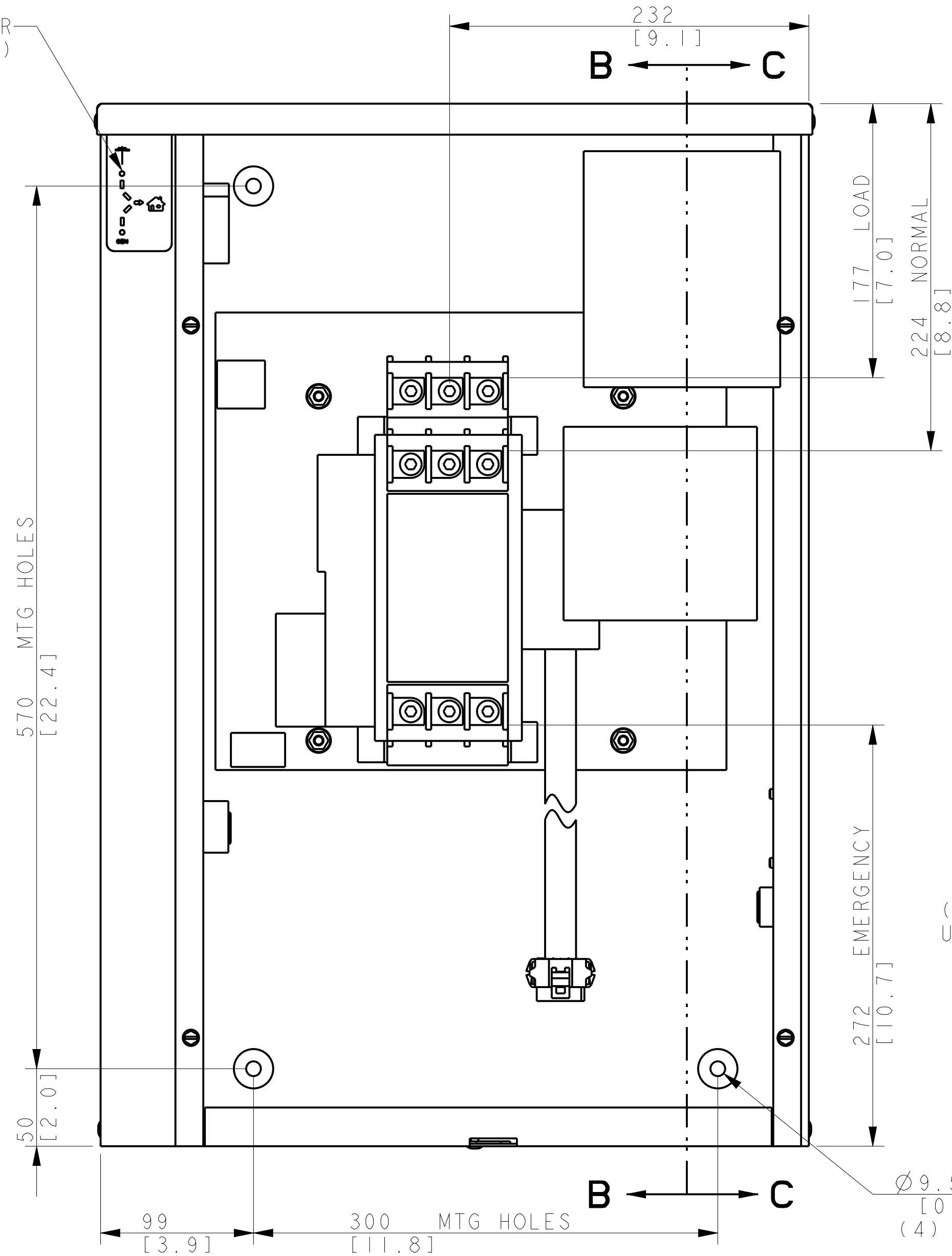
100/200A CONTACTOR (COVER REMOVED TO SHOW DETAIL)
