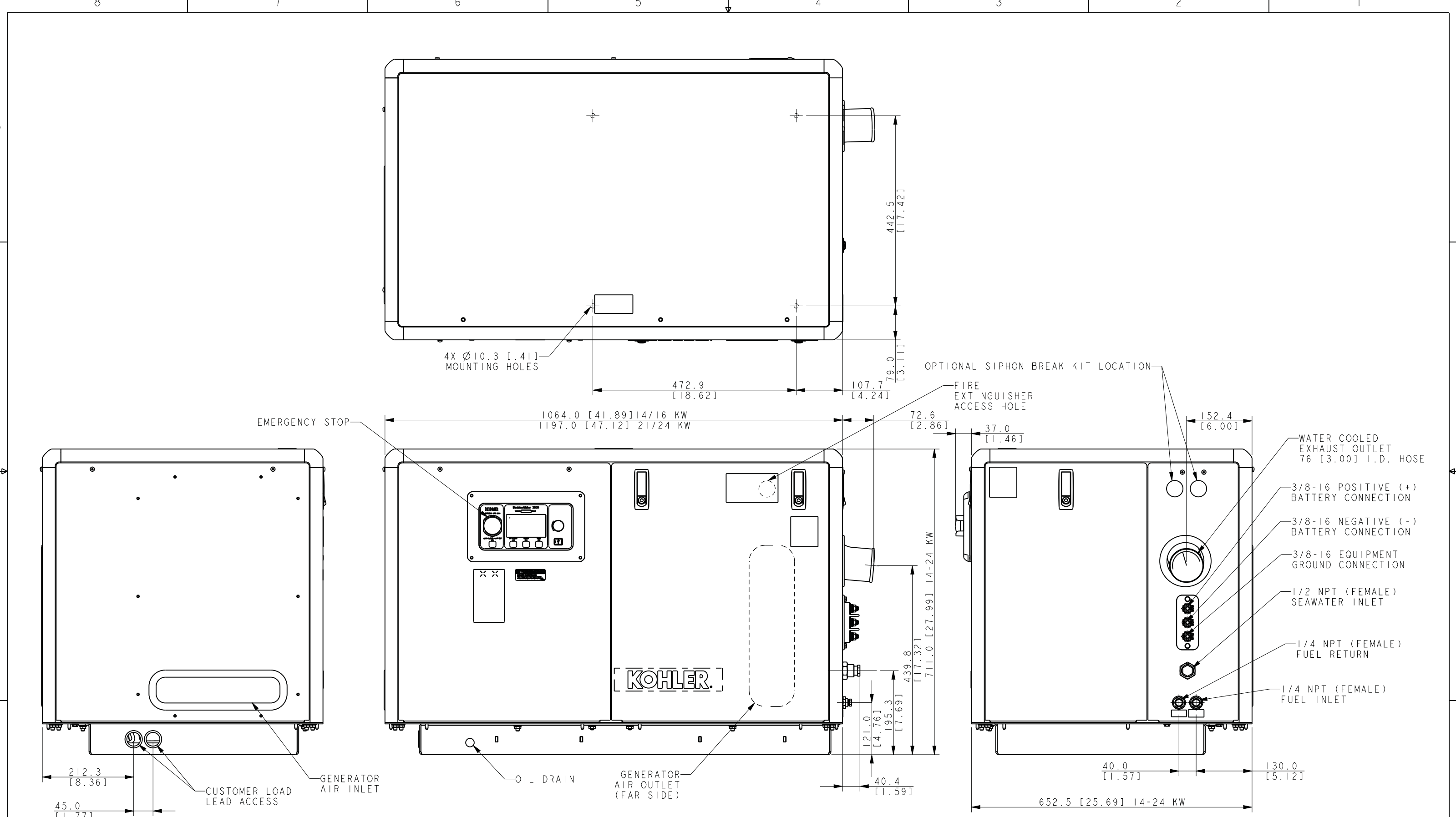
SOUND SHIELD WITH FRONT CONNECTION PANEL
