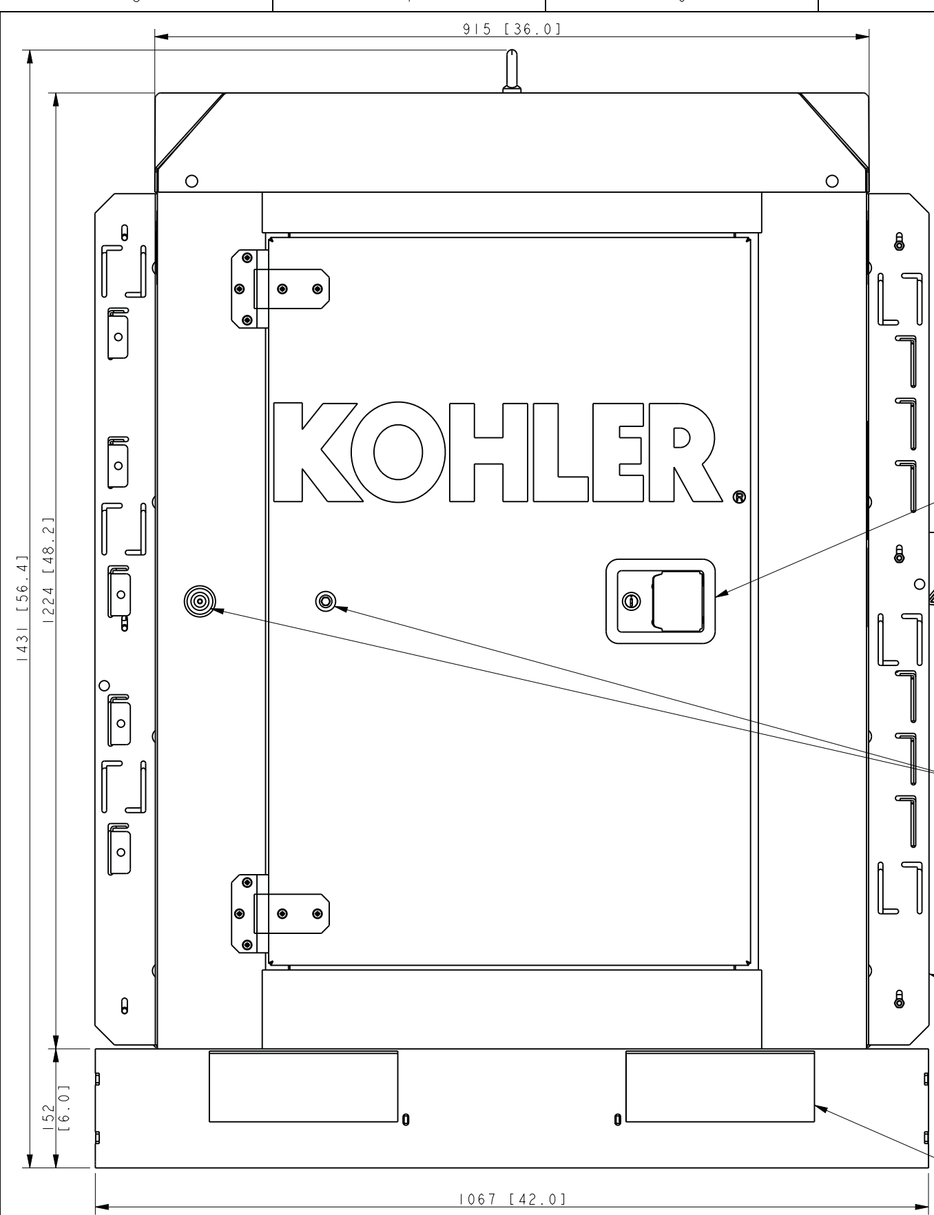
FRONT VIEW
