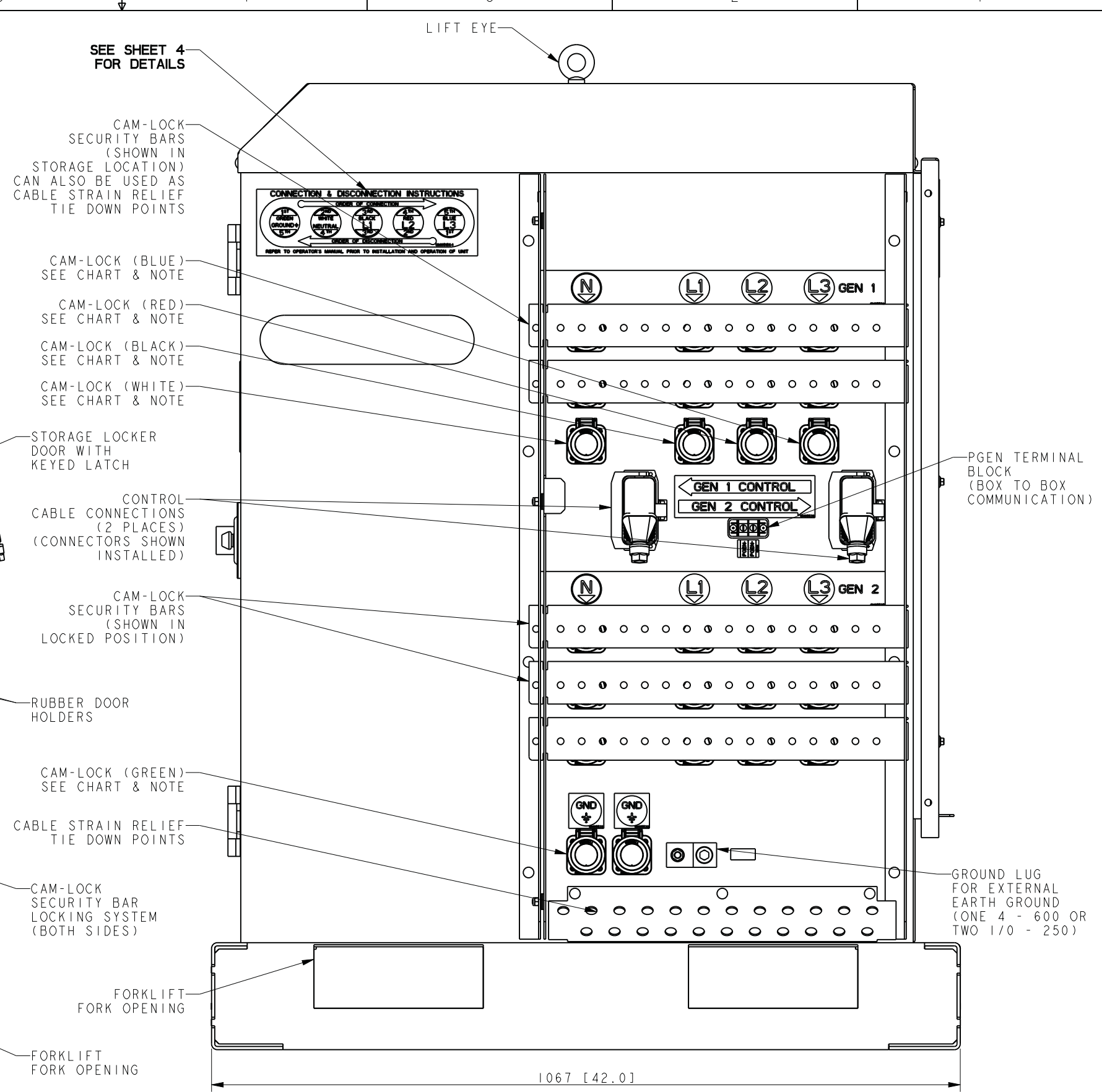
RIGHT SIDE VIEW
