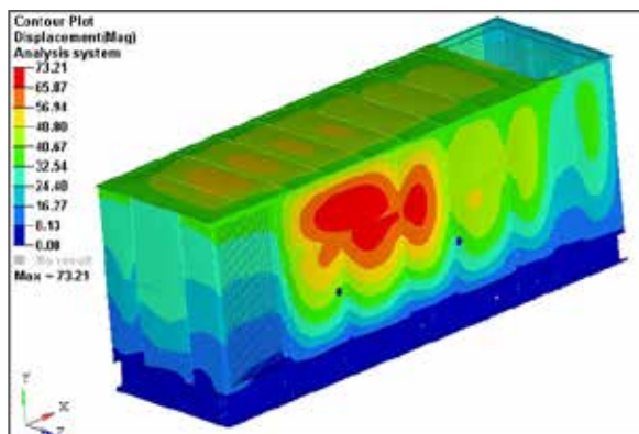
Figure 4: Analytical Deflection Plot Due to Basic Wind Speed Load on Enclosure Source: Kohler Power Systems
