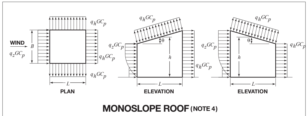
Figure 3. Typical External Pressure Profiles Source: ASCE 7-05
